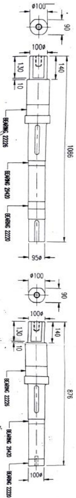
DETAIL OF DRIVE SHAFT FOR P10 SCREW PRESS WITH FLATHEAD AT SCREW END (PART NO: 4B-C)
